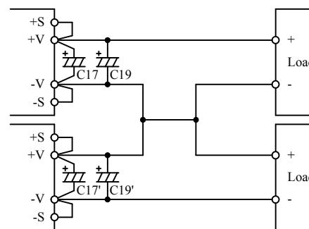
Fig.6-11 Series operation ±output series applications
