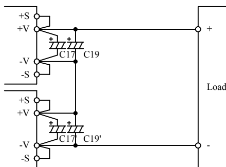
Fig.6-10 Series operation for high output voltage applications
