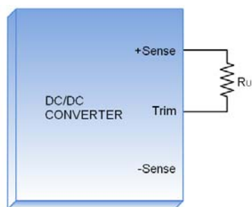
TRIM-UP
