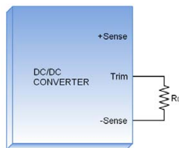
TRIM-DOWN
